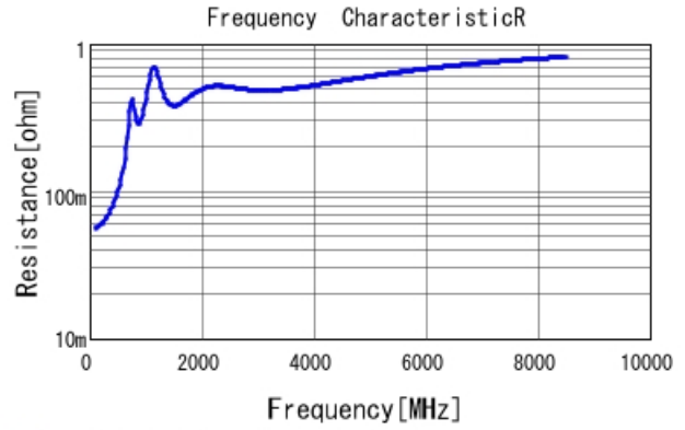
■ GCM1555C1H621FA16 R DCOV, 25degC
