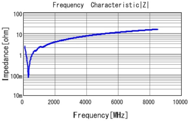
■ GCM1555C1H621FA16 |Z| DCOV, 25degC
