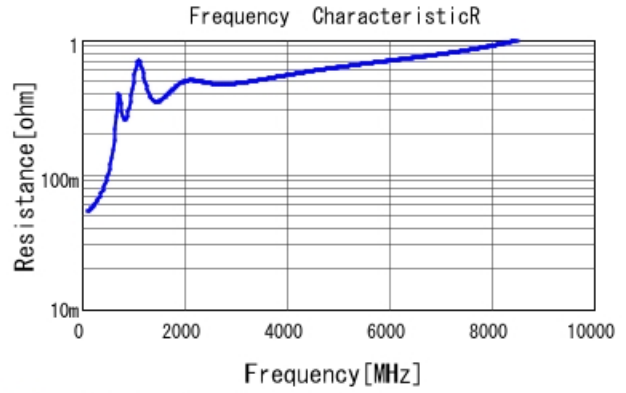
GCM1555C1H681FA16 R DCOV, 25degC
