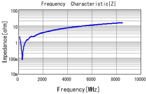
GCM1555C1H681FA16 |Z| DCOV, 25degC
