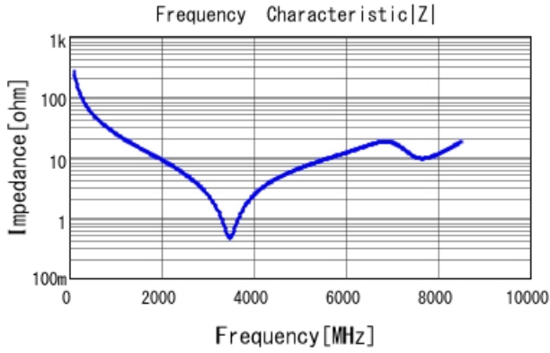
■ GCM1555C1H6R0CA16 |Z| DCOV, 25degC
