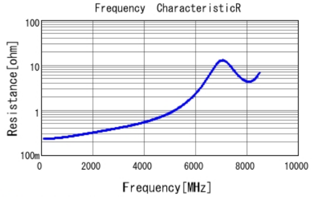
■ GCM1555C1H6R0FA16 R DCOV, 25degC
