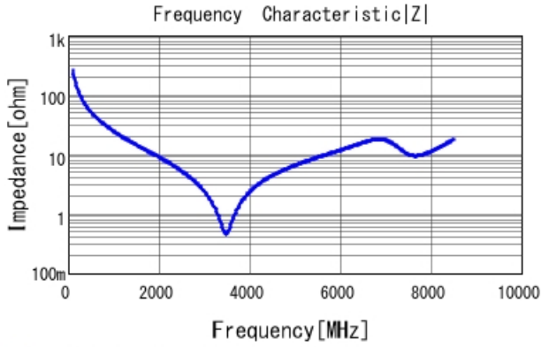
■ GCM1555C1H6R0FA16 |Z| DCOV, 25degC
