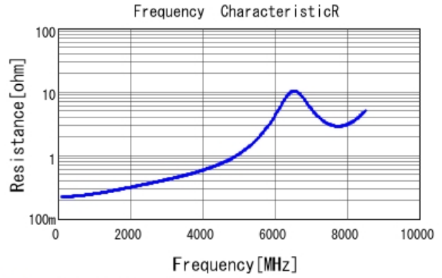
■ GCM1555C1H7R0WA16 R DCOV, 25degC
