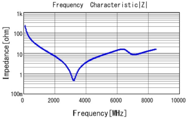
■ GCM1555C1H7R0WA16 |Z| DCOV, 25degC
