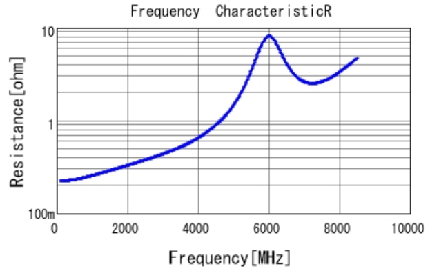
■ GCM1555C1H8R0CA16 R DCOV, 25degC
