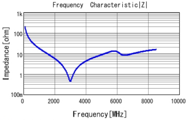
■ GCM1555C1H8R0CA16 |Z| DCOV, 25degC
