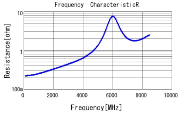
GCM1555C1H8R2BA16 R DC0V, 25degC
