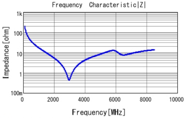
GCM1555C1H8R2BA16 |Z| DC0V, 25degC
