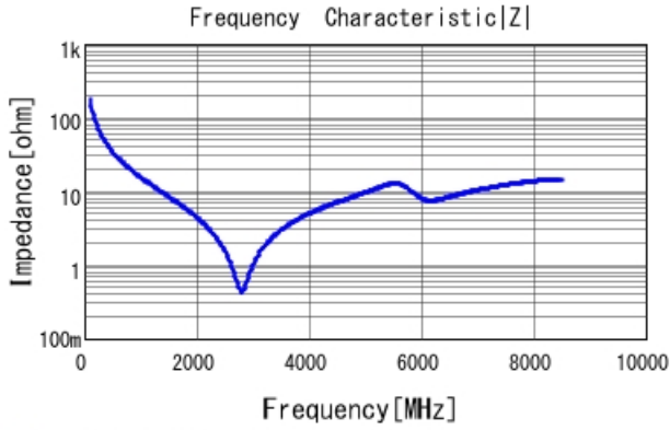
GCM1555C1H9R0WA16 |Z| DCOV, 25degC
