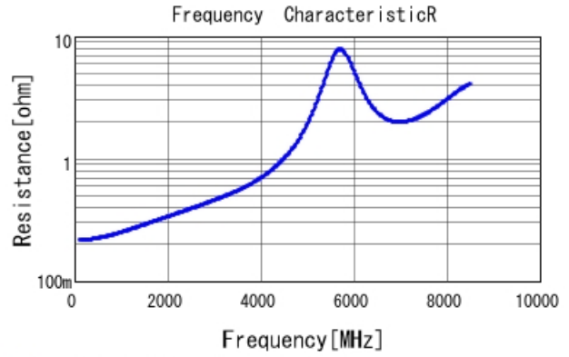
GCM1555C1H9R0WA16 R DCOV, 25degC
