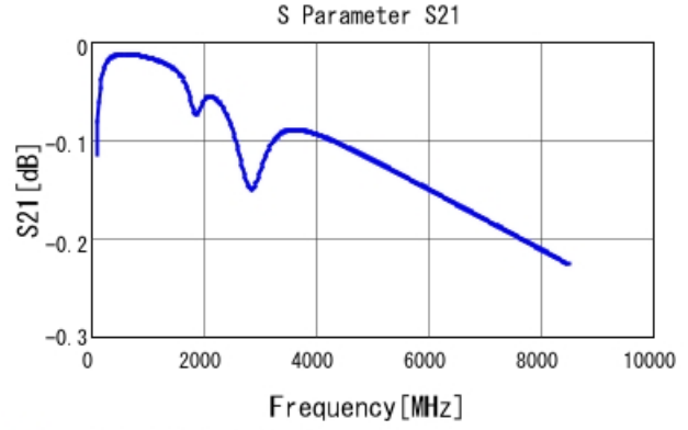
■ GCM1555G1H101FA16 S21 DCOV, 25degC
