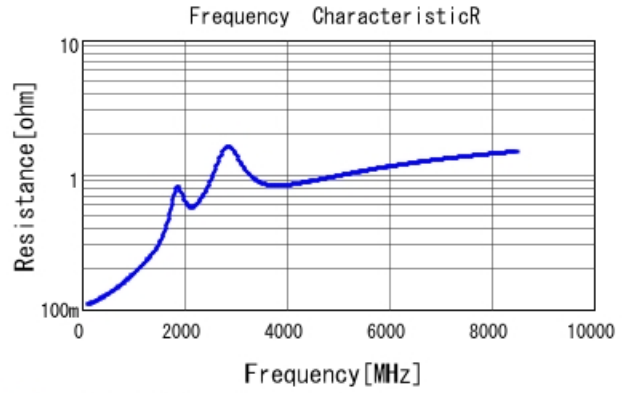
■ GCM1555G1H101FA16 R DC0V, 25degC
