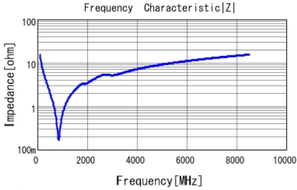
■ GCM1555G1H101FA16 |Z| DC0V, 25degC
