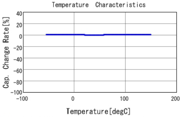
■ GCM1555G1H1R0CA16 C-Temp. capchange, DCOV, AC1Vrms
