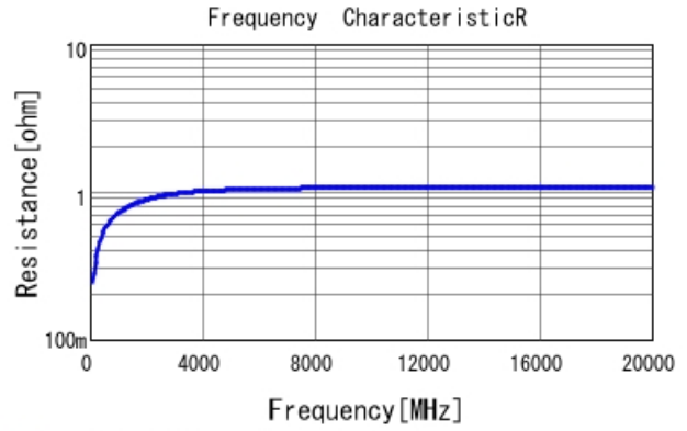
GCM1555G1H1R0CA16 R DCOV, 25degC
