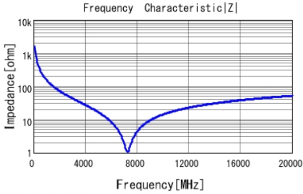
GCM1555G1H1R0CA16 |Z| DCOV, 25degC
