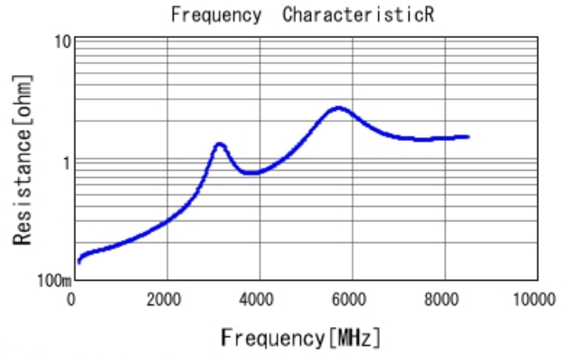
■ GCM1555G1H330FA16 R DC0V, 25degC
