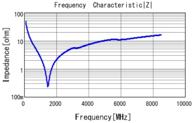
■ GCM1555G1H330FA16 |Z| DC0V, 25degC
