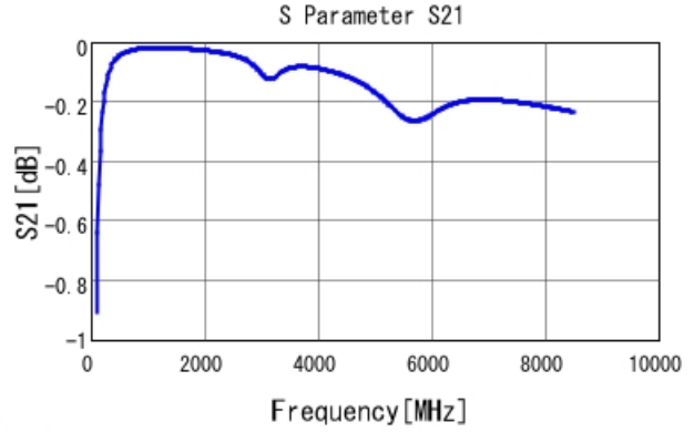
■ GCM1555G1H330FA16 S21 DCOV, 25degC
