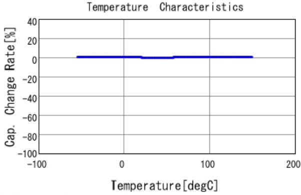
■ GCM1555G1H330FA16 C-Temp. capchange, DCOV, AC1Vrms
