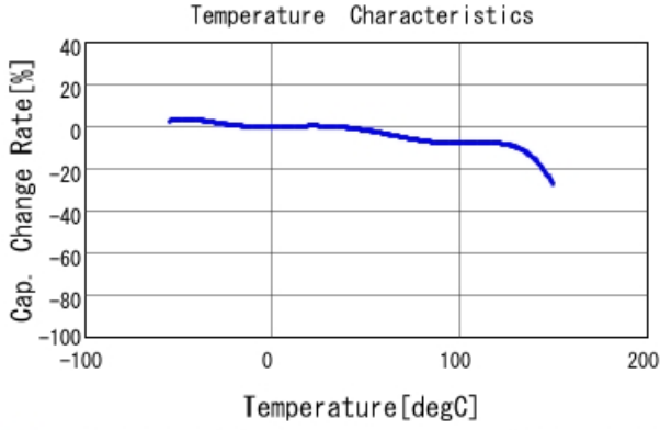
■ GCM155L81H472KA37 C-Temp. capchange, DCO. 0V, AC1. 0Vrm
