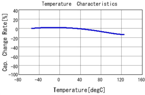
■ GCM155R71C683KA55 C-Temp. capchange, DCO. 0V, AC1.0V rm
