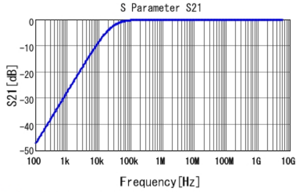
■ GCM155R71C683KA55 S21 DCOV, 25degC
