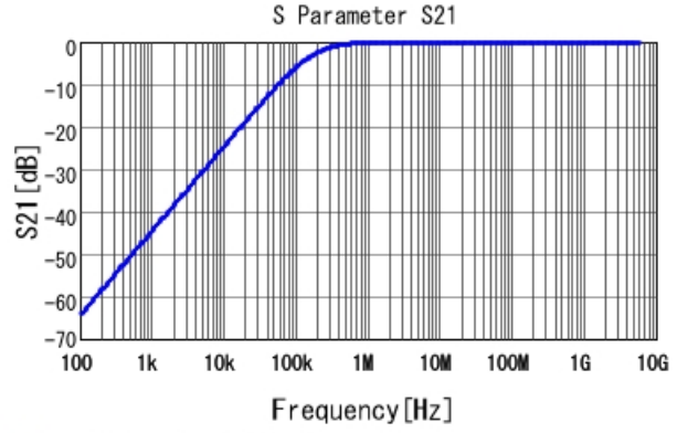
■ GCM155R71E103KA37 S21 DCOV, 25degC
