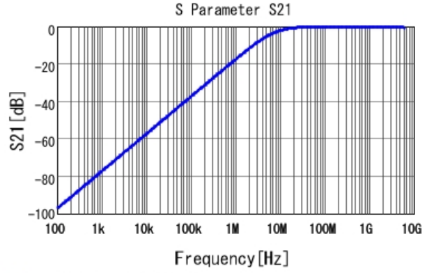
■ GCM155R71H221KA37 S21 DCOV, 25degC
