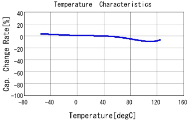
■ GCM155R71H332KA37 C-Temp. capchange, DCO. 0V, AC1. 0Vrm
