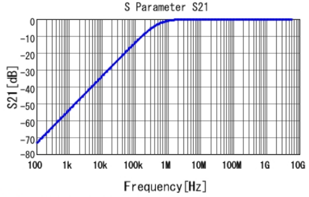
■ GCM155R71H332KA37 S21 DCOV, 25degC
