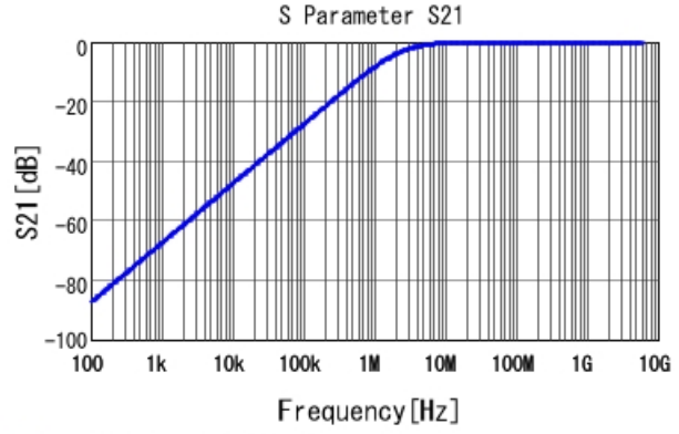
■ GCM155R71H681KA37 S21 DCOV, 25degC
