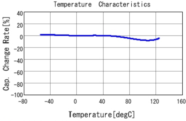
■ GCM155R71H681KA37 C-Temp. capchange, DCO. 0V, AC1.0Vrm
