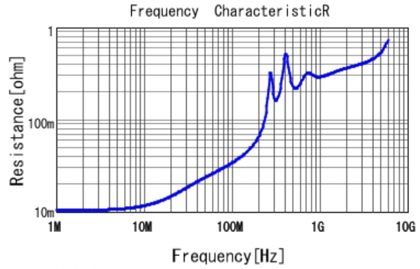
■ GCM1885C1H272JA16 R DCOV, 25degC
