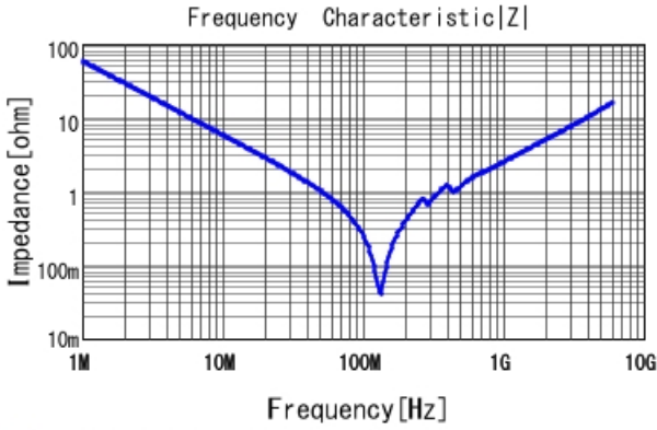
■ GCM1885C1H272JA16 |Z| DCOV, 25degC
