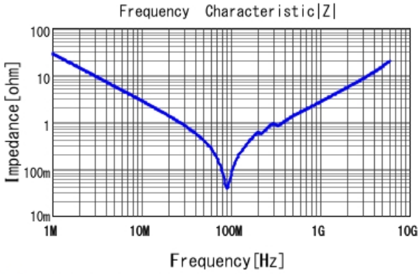
GCM1885C1H562JA16 |Z| DCOV, 25degC
