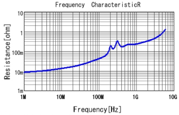
GCM1885C1H562JA16 R DCOV, 25degC
