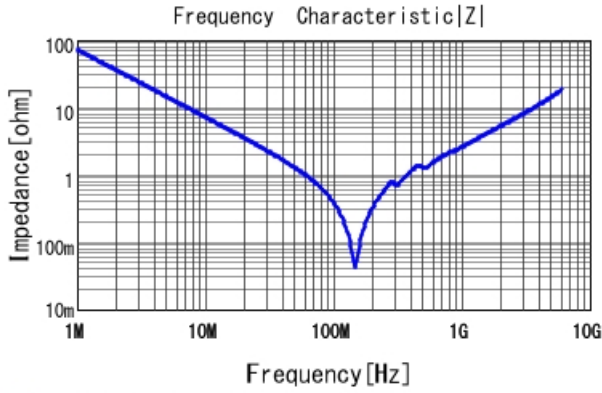
GCM1885C1J222JA16 |Z| DCOV, 25degC
