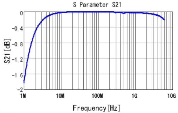
■ GCM1885C1J222JA16 S21 DCOV, 25degC
