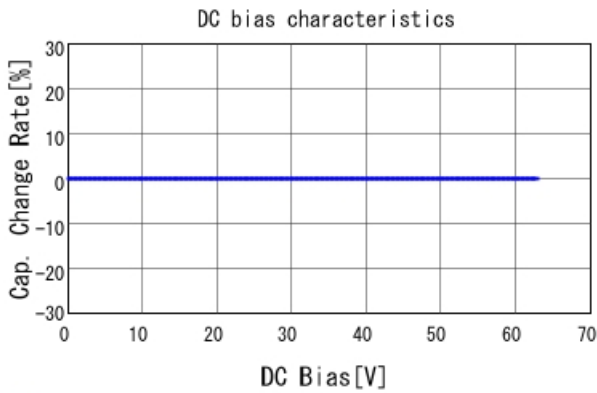
GCM1885C1J222JA16 C-DC bias capchange, 25.0degC, AC1V
