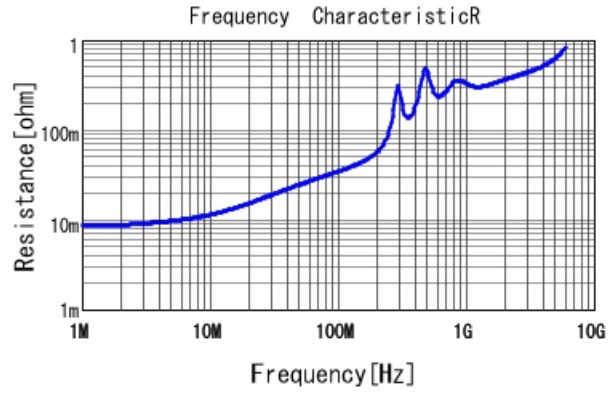
GCM1885C1J222JA16 R DCOV, 25degC
