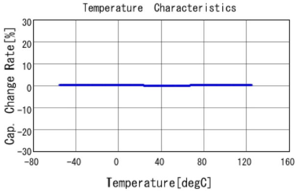
■ GCM1885C1J222JA16 C-Temp. capchange, DCOV, AC1Vrms
