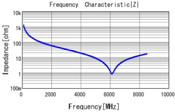
GCM1885C2A1R2BA16 |Z| DCOV, 25degC
