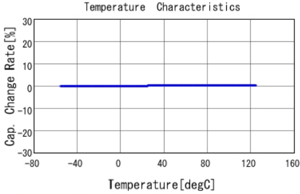
■ GCM1885C2A1R2BA16 C-Temp. capchange, DCOV, AC1Vrms
