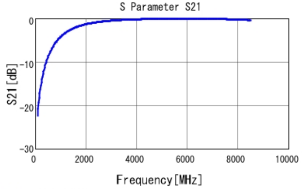
■ GCM1885C2A1R2BA16 S21 DCOV, 25degC
