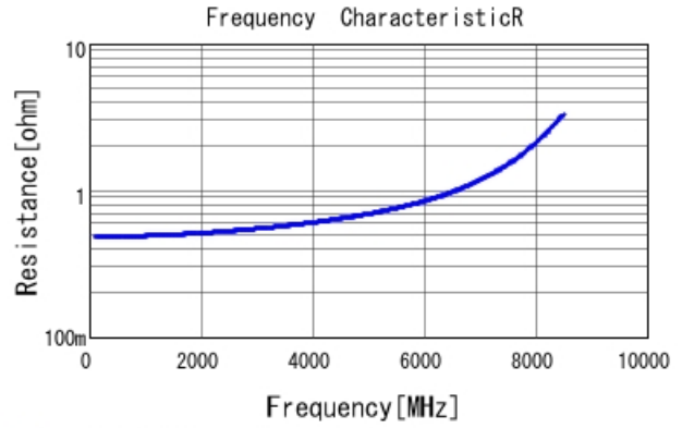
GCM1885C2A1R2BA16 R DCOV, 25degC
