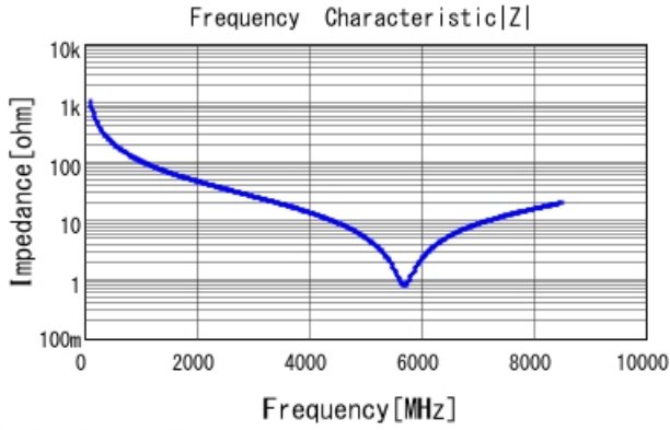
GCM1885C2A1R5BA16 |Z| DC0V, 25degC
