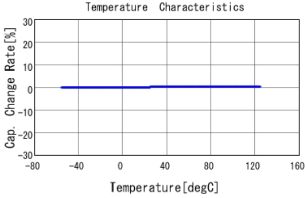
■ GCM1885C2A1R5BA16 C-Temp. capchange, DCOV, AC1Vrms
