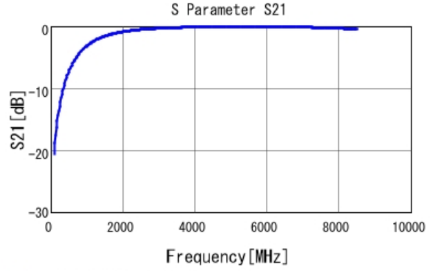
■ GCM1885C2A1R5BA16 S21 DCOV, 25degC
