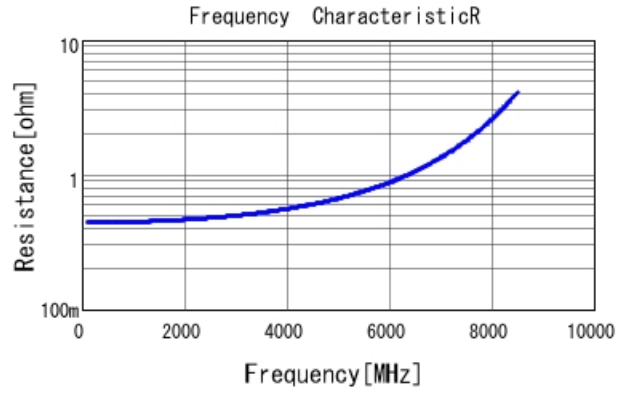
GCM1885C2A1R5BA16 R DC0V, 25degC
