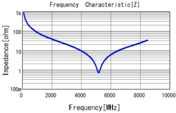
GCM1885C2A1R8BA16 |Z| DCOV, 25degC
