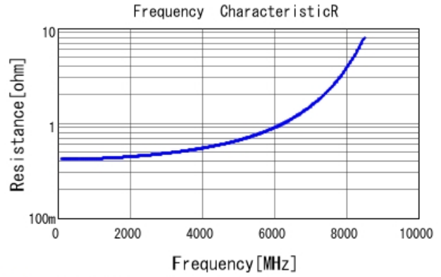
GCM1885C2A1R8BA16 R DCOV, 25degC
