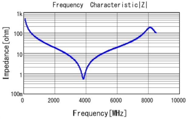
■ GCM1885C2A3R3BA16 |Z| DCOV, 25degC
