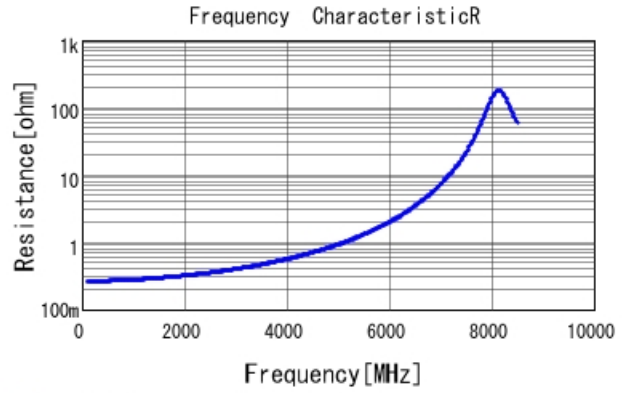
■ GCM1885C2A3R3BA16 R DCOV, 25degC
