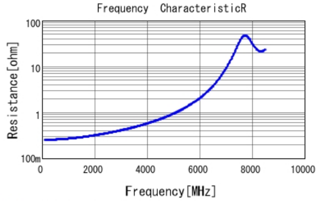
GCM1885C2A3R9BA16 R DCOV, 25degC
