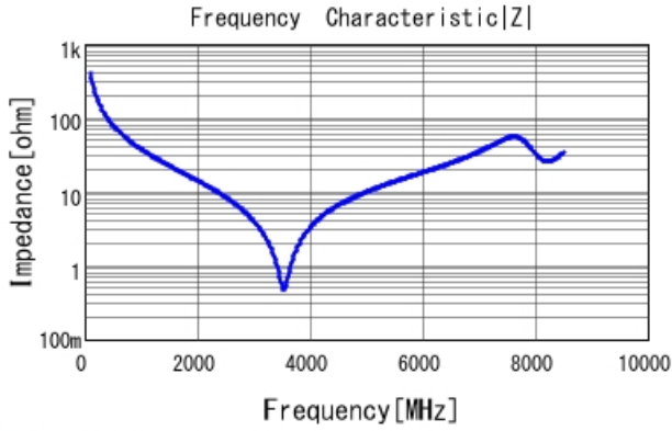
GCM1885C2A3R9BA16 |Z| DCOV, 25degC
