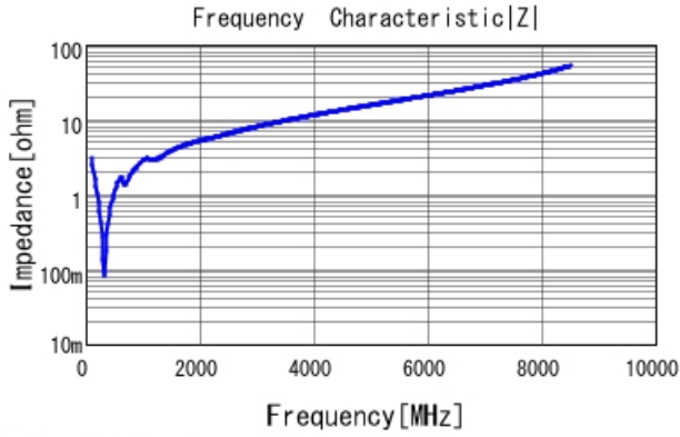
■ GCM1885C2A471JA16 |Z| DCOV, 25degC
