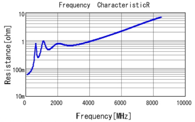
■ GCM1885C2A471JA16 R DCOV, 25degC
