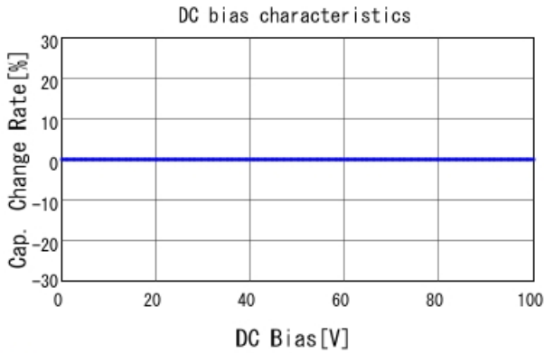
■ GCM1885C2A471JA16 C-DC bias capchange, 25.0degC, AC1V
