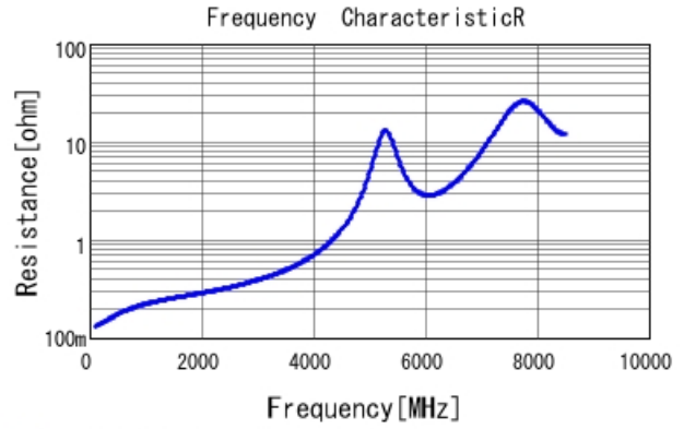
■ GCM1885C2A8R0DA16 R DCOV, 25degC
