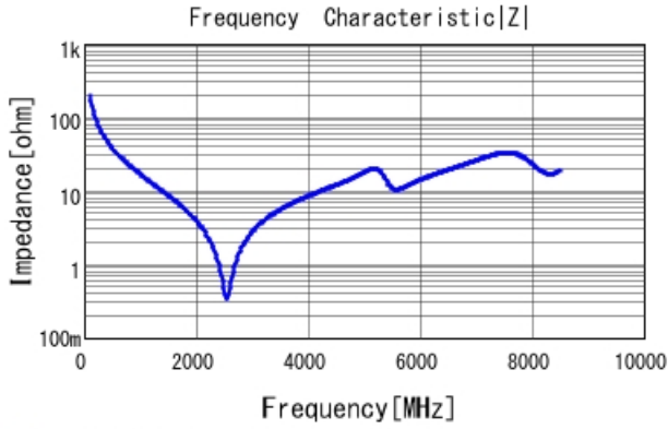
■ GCM1885C2A8R0DA16 |Z| DCOV, 25degC
