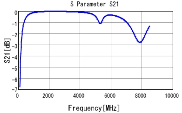
■ GCM1885C2A8R2BA16 S21 DCOV, 25degC
