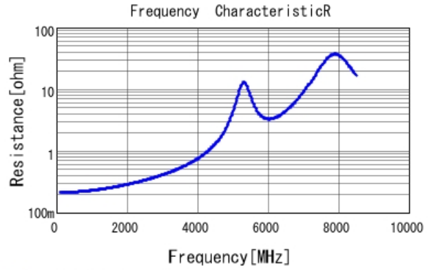
■ GCM1885C2A8R2BA16 R DCOV, 25degC
