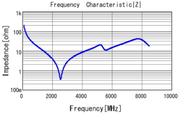
■ GCM1885C2A8R2BA16 |Z| DCOV, 25degC
