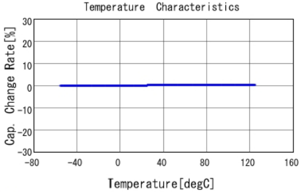
■ GCM1885C2A8R2BA16 C-Temp. capchange, DCOV, AC1Vrms
