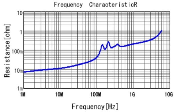
■ GCM1887U1H103JA16 R DCOV, 25degC
