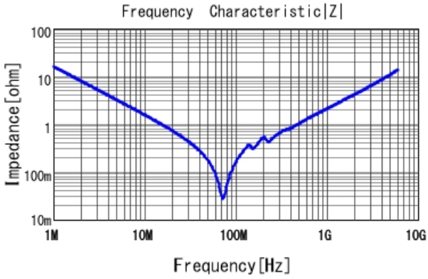
■ GCM1887U1H103JA16 |Z| DCOV, 25degC
