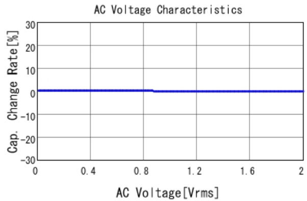
■ GCM1887U1H103JA16 C-AC Voltage capchange, DCOV, 25.0d
