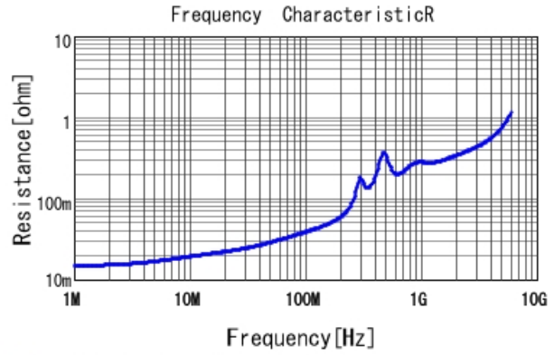
GCM1887U1H332JA16 R DCOV, 25degC
