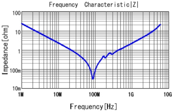
■ GCM1887U1H682JA16 |Z| DCOV, 25degC
