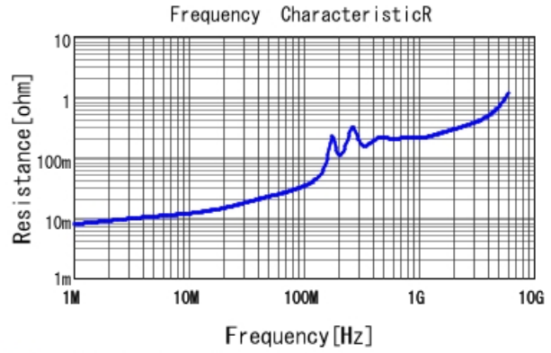
■ GCM1887U1H682JA16 R DCOV, 25degC
