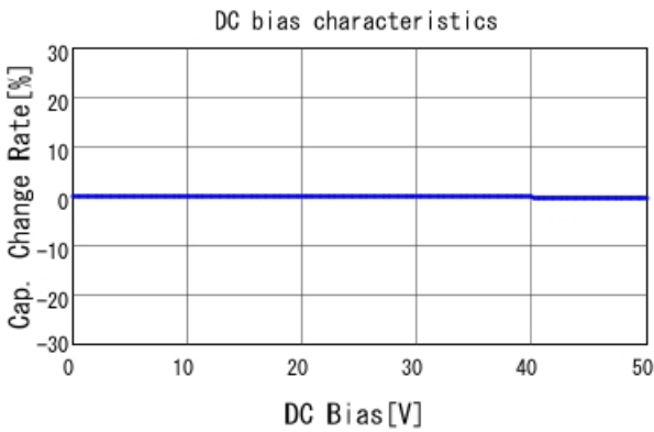
■ GCM1887U1H682JA16 C-DC bias capchange, 25.0degC, AC1V
