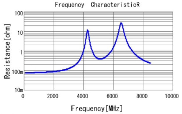
■ GJM1555C1H220JB01 R DC0V, 25degC
