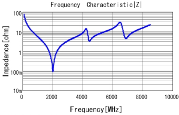
■ GJM1555C1H220JB01 |Z| DC0V, 25degC
