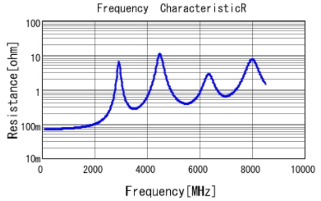
■ GJM1555C1H470JB01 R DC0V, 25degC
