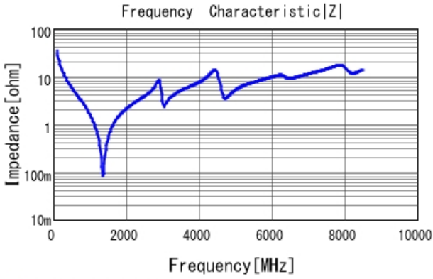
■ GJM1555C1H470JB01 |Z| DC0V, 25degC
