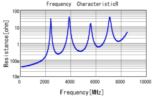
■ GQM2195G2E470JB12 R DC0V, 25degC
