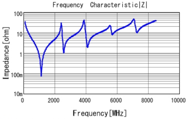
■ GQM2195G2E470JB12 |Z| DC0V, 25degC
