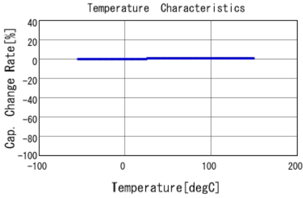
■ GQM2195G2E470JB12 C-Temp. capchange, DCOV, AC1Vrms
