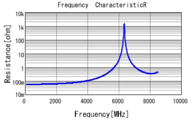
■ GQM22M5C2H3R9CB01 R DC0V, 25degC
