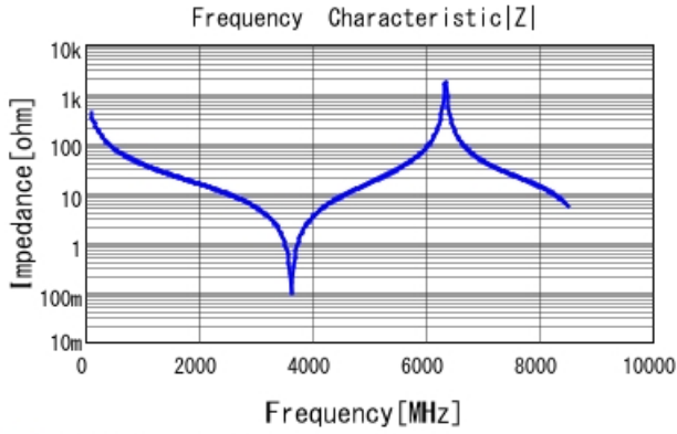
■ GQM22M5C2H3R9CB01 |Z| DC0V, 25degC
