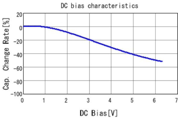
■ GRJ188C70J475KE11 C-DC bias capchange, 25.0degC, AC1V
