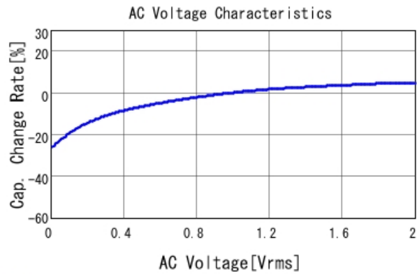
■ GRJ188C70J475KE11 C-AC Voltage capchange, DC0V, 25.0d
