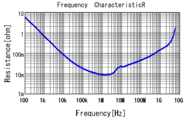
■ GRJ188C70J475KE11 R DC0V, 25degC
