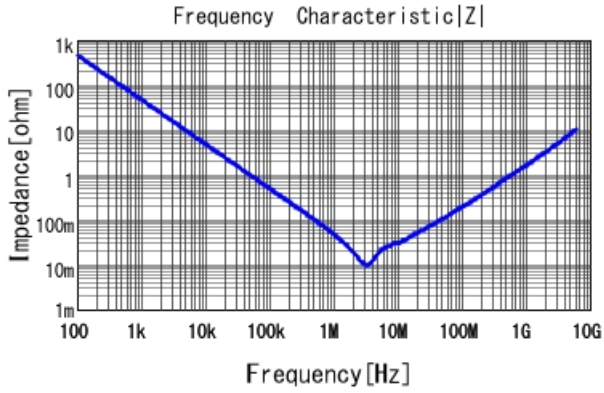
■ GRJ188C70J475KE11 |Z| DC0V, 25degC
