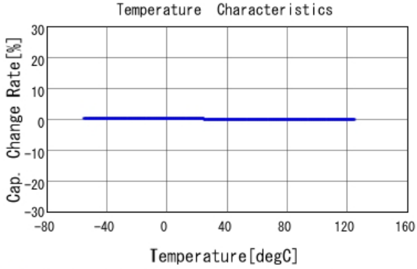
■ GRM0335C1E220JA01 C-Temp. capchange, DCOV, AC1Vrms
