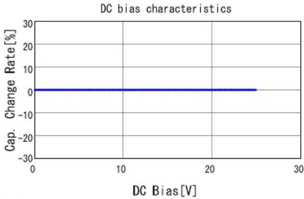
■ GRM0335C1E220JA01 C-DC bias capchange, 25.0degC, AC1V
