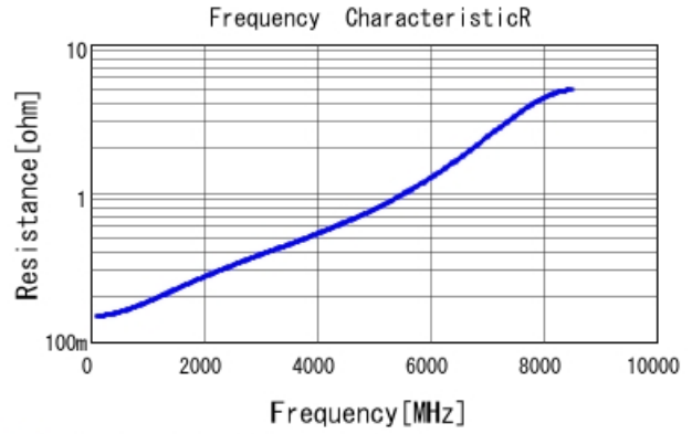
■ GRM0335C1E220JA01 R DCOV, 25degC
