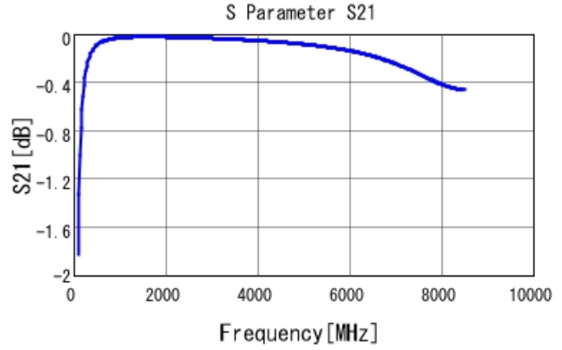
■ GRM0335C1E220JA01 S21 DCOV, 25degC
