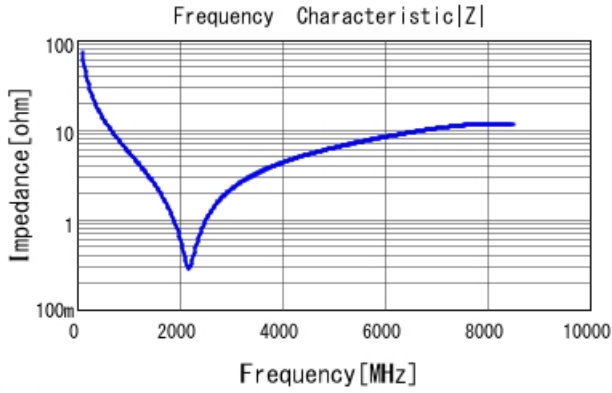
■ GRM0335C1E220JA01 |Z| DCOV, 25degC
