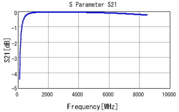
■ GRM0335C1H120GA01 S21 DCOV, 25degC
