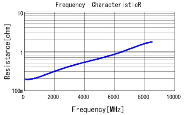
■ GRM0335C1H120GA01 R DCOV, 25degC
