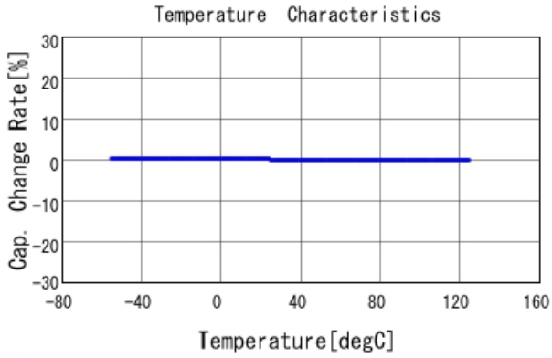
■ GRM0335C1H120GA01 C-Temp. capchange, DCOV, AC1Vrms
