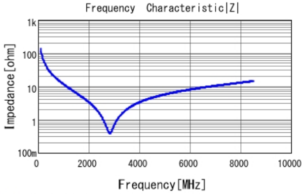
■ GRM0335C1H120GA01 |Z| DCOV, 25degC
