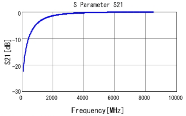
■ GRM0335C1H1R2BA01 S21 DCOV, 25degC
