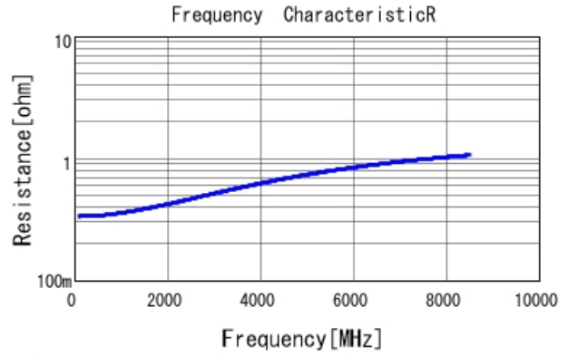
■ GRM0335C1H1R2BA01 R DCOV, 25degC
