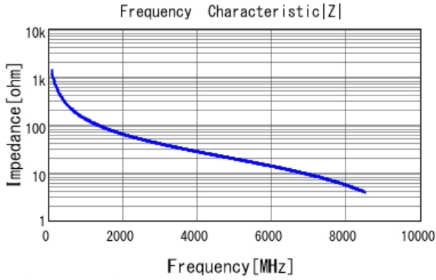
■ GRM0335C1H1R2BA01 |Z| DCOV, 25degC
