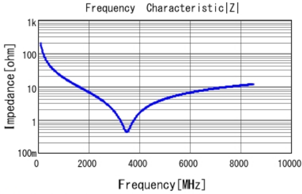
■ GRM0335C1H8R0DA01 |Z| DCOV, 25degC
