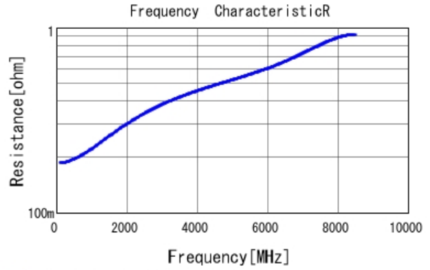
■ GRM0335C1H8R0DA01 R DCOV, 25degC
