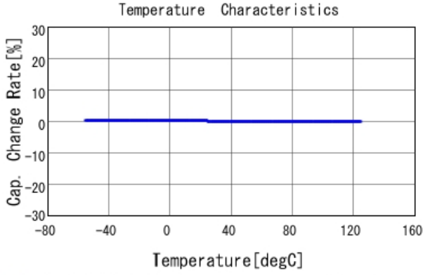
■ GRM0335C2A1R3WA01 C-Temp. capchange, DCOV, AC1Vrms
