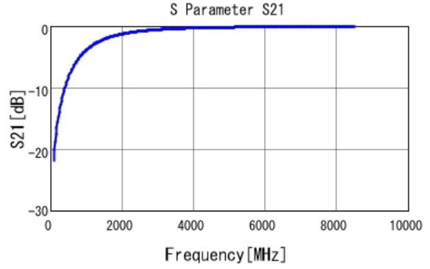
■ GRM0335C2A1R3WA01 S21 DCOV, 25degC
