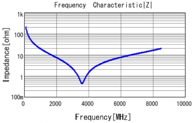
■ GRM0335C2A7R6WA01 |Z| DCOV, 25degC
