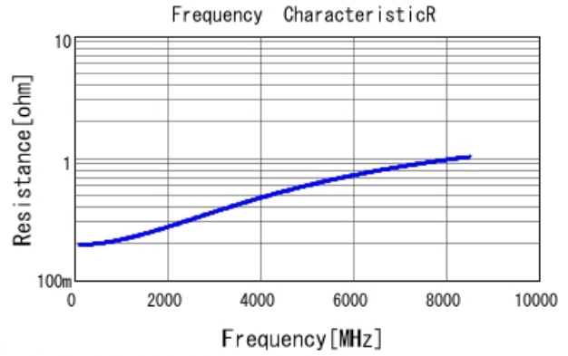
■ GRM0335C2A7R6WA01 R DCOV, 25degC
