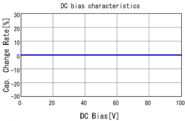
■ GRM0335C2A7R6WA01 C-DC bias capchange, 25.0degC, AC1V
