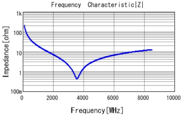
■ GRM0335C2A7R7DA01 |Z| DCOV, 25degC
