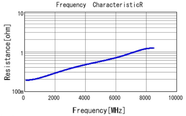
■ GRM0335C2A7R7DA01 R DCOV, 25degC
