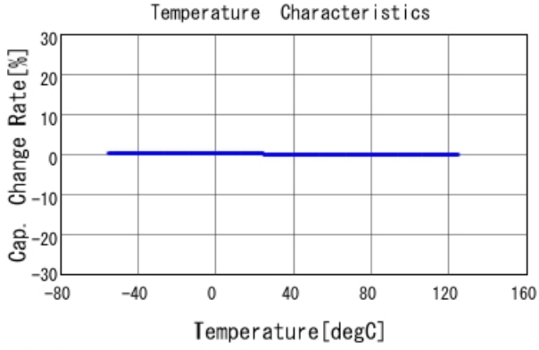
■ GRM0335C2AR90WA01 C-Temp. capchange, DCOV, AC1Vrms
