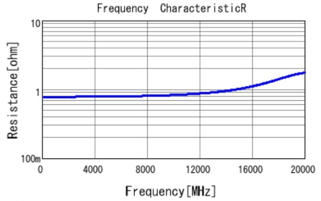
■ GRM0335C2AR90WA01 R DCOV, 25degC
