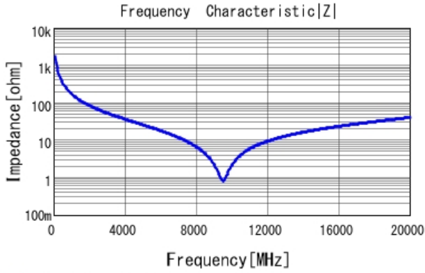
■ GRM0335C2AR90WA01 |Z| DCOV, 25degC
