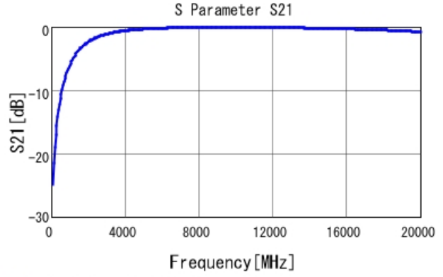
■ GRM0335C2AR90WA01 S21 DCOV, 25degC
