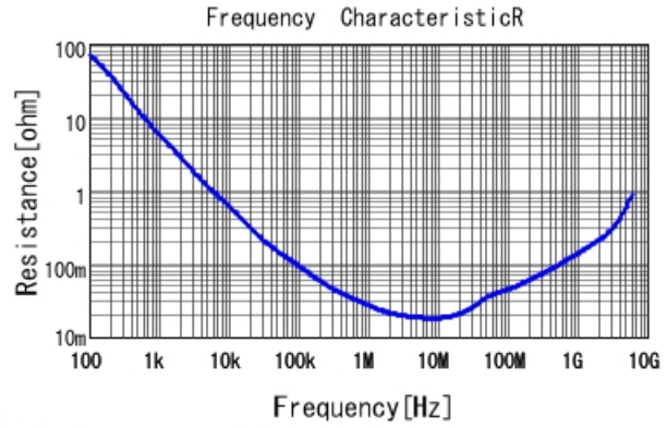
■ GRM033C80J224KE90 R DCOV, 25degC
