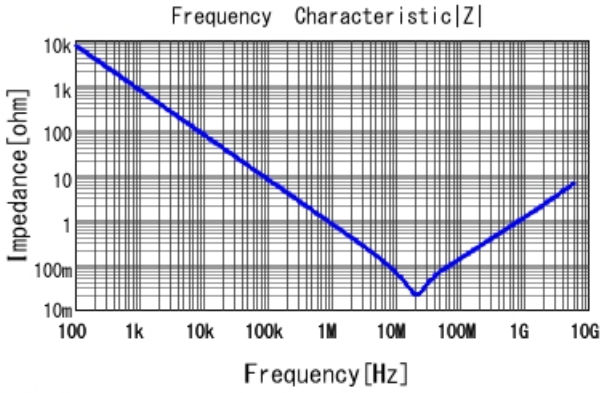
■ GRM033C80J224KE90 |Z| DCOV, 25degC
