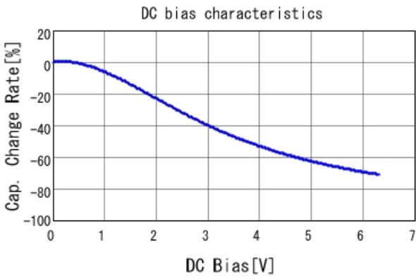
■ GRM033C80J224KE90 C-DC bias capchange, 25.0degC, AC0.
