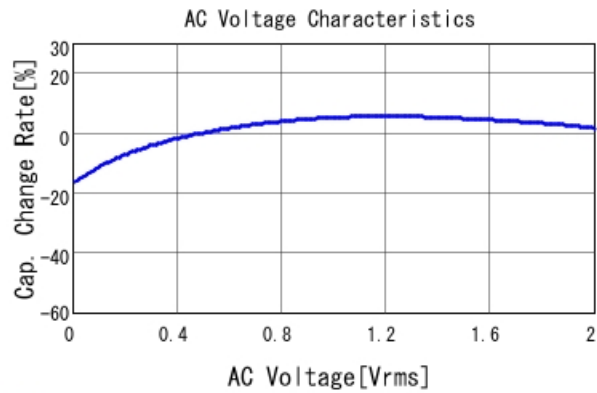
■ GRM033C80J224KE90 C-AC Voltage capchange, DCOV, 25.0d
