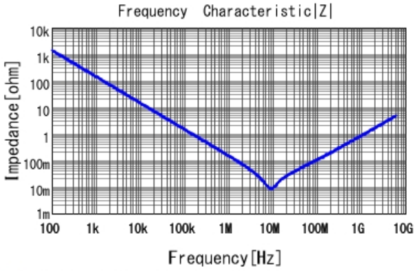
■ GRM033R60J155ME14 |Z| DCOV, 25degC
