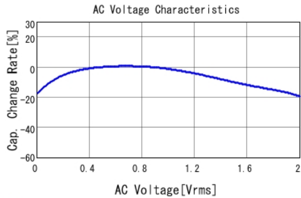
■ GRM033R60J155ME14 C-AC Voltage capchange, DCOV, 25.0d
