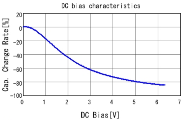
■ GRM033R60J155ME14 C-DC bias capchange, 25.0degC, AC0.
