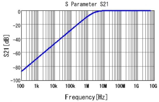
■ GRM033R71E681KA01 S21 DCOV, 25degC
