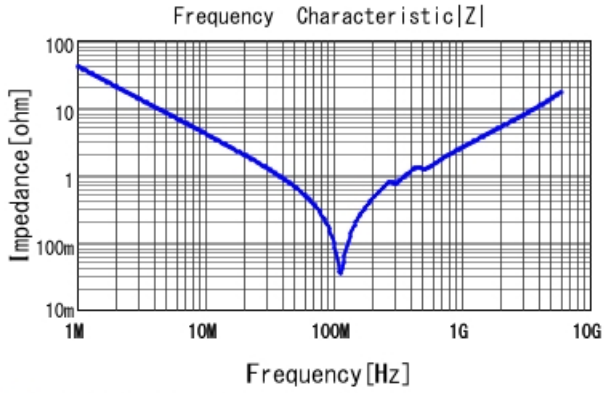
■ GRM2165C2A392JA01 |Z| DCOV, 25degC
