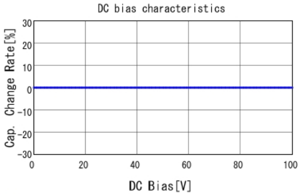
■ GRM2165C2A392JA01 C-DC bias capchange, 25.0degC, AC1V
