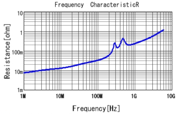
■ GRM2165C2A392JA01 R DCOV, 25degC
