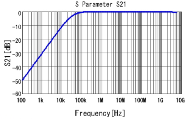
■ GRM21BR72A473KA01 S21 DCOV, 25degC
