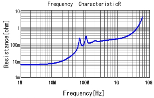
■ GRM3195C1H333JA01 R DCOV, 25degC
