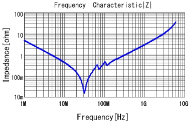
■ GRM3195C1H333JA01 |Z| DCOV, 25degC
